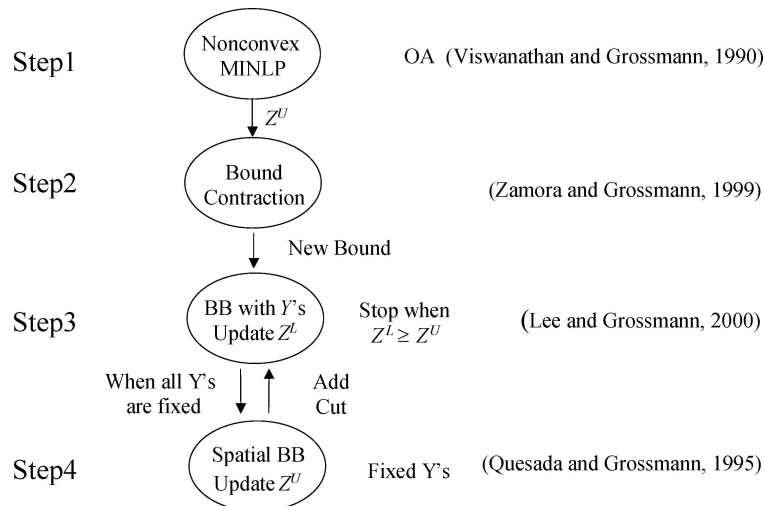
Figure 7. Global optimization algorithm for nonconvex GDP.
