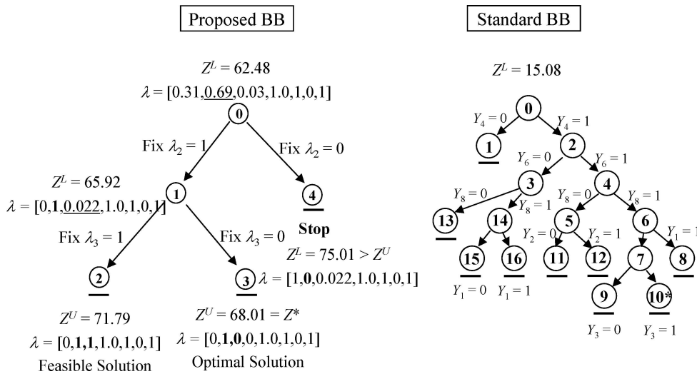
Figure 6. Comparison of branch and bound methods.
