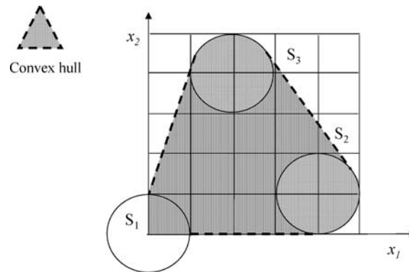
Figure 1. Feasible set and convex hull of Example 1.
