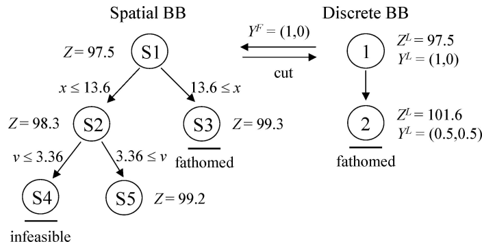
Figure 8. Branch and bound tree for nonconvex GDP example.
