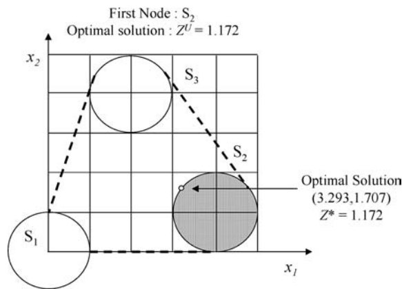
Figure 2. Feasible set at the first node.
