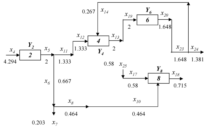
Figure 5. The optimal plant structure.
