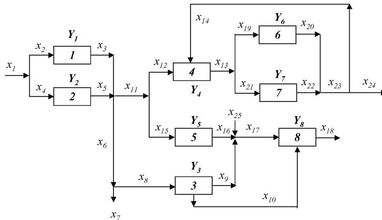
Figure 4. Superstructure for process network example.
