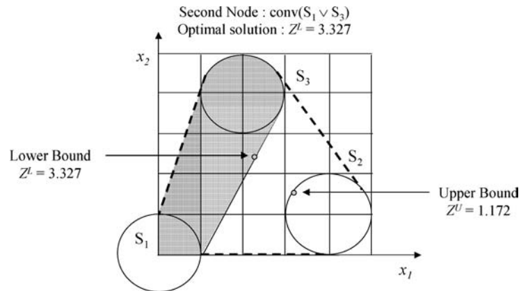
Figure 3. Feasible set at the second node.
